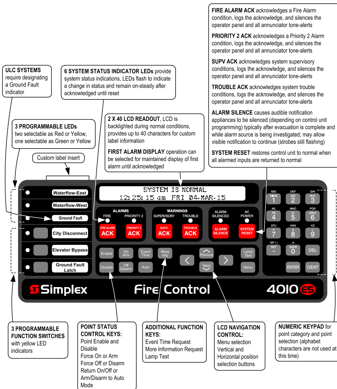
Figure 9: Operator Interface Features
