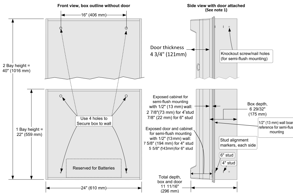
Figure 11: Cabinet dimension reference
