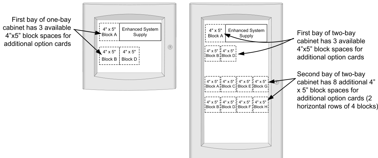
Figure 10: Cabinet One and Two Bay Loading Reference
