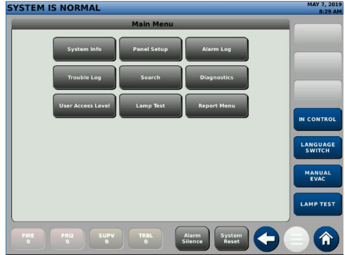
Figure 8: Main Menu
