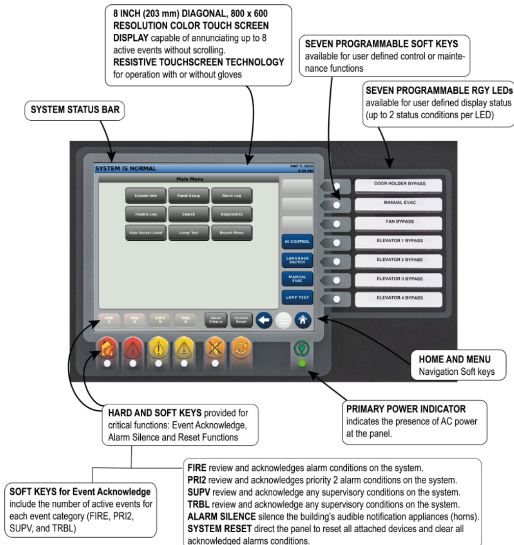
Figure 6: ES Touch Screen Display Operator Interface
