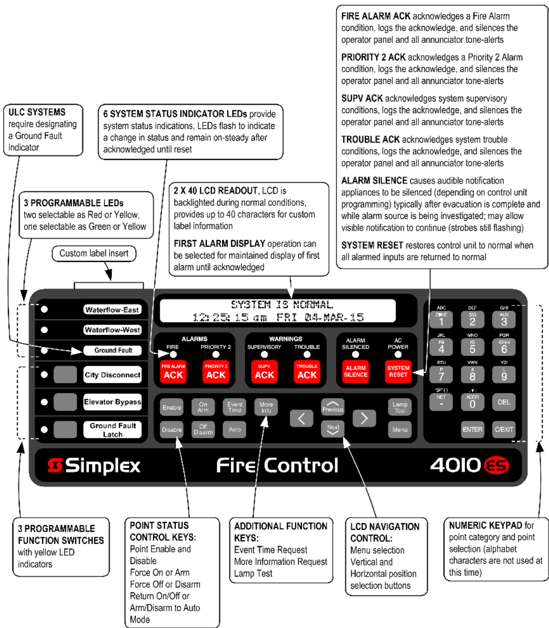
Figure 13: Operator Interface Features
