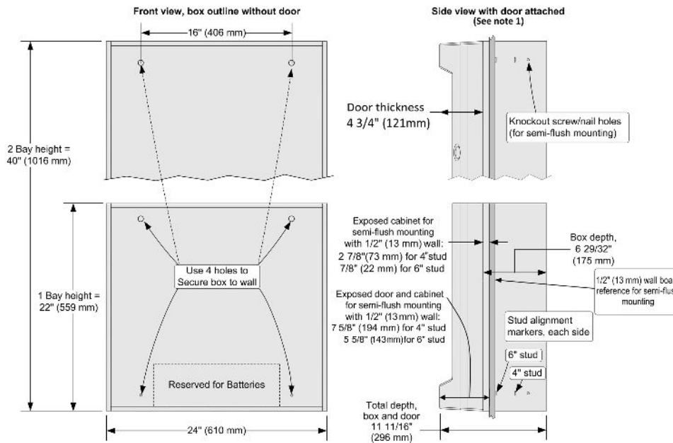
Figure 15: Cabinet dimension reference
